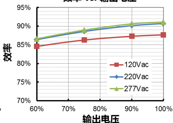
EUP-200S350SV( I_o=3500mA )
