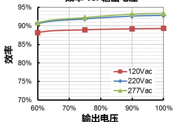
EUP-200S350SV( I_o=2450mA )
