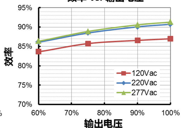
EUP-200S350SV( I_o=3500mA )
