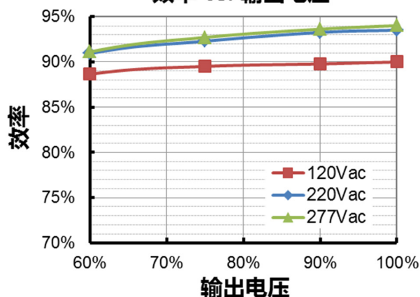
EUP-200S210SV( I_o=1400mA )
