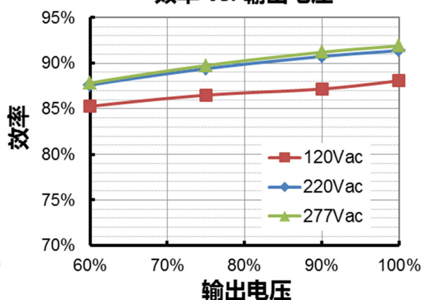
EUP-200S210SV( I_o=2100mA )
