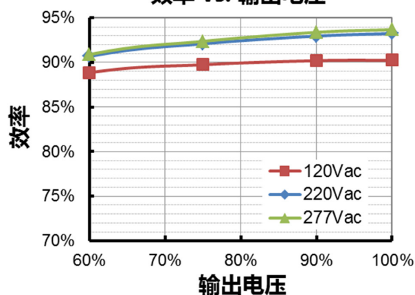
EUP-200S350SV( I_o=2450mA )
